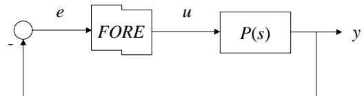
Fig. 3. Block diagram of a reset control system with FORE.
