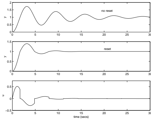
Fig. 2. Step response y of the linear control system (top), reset control system (middle) and reset control action u (bottom).
